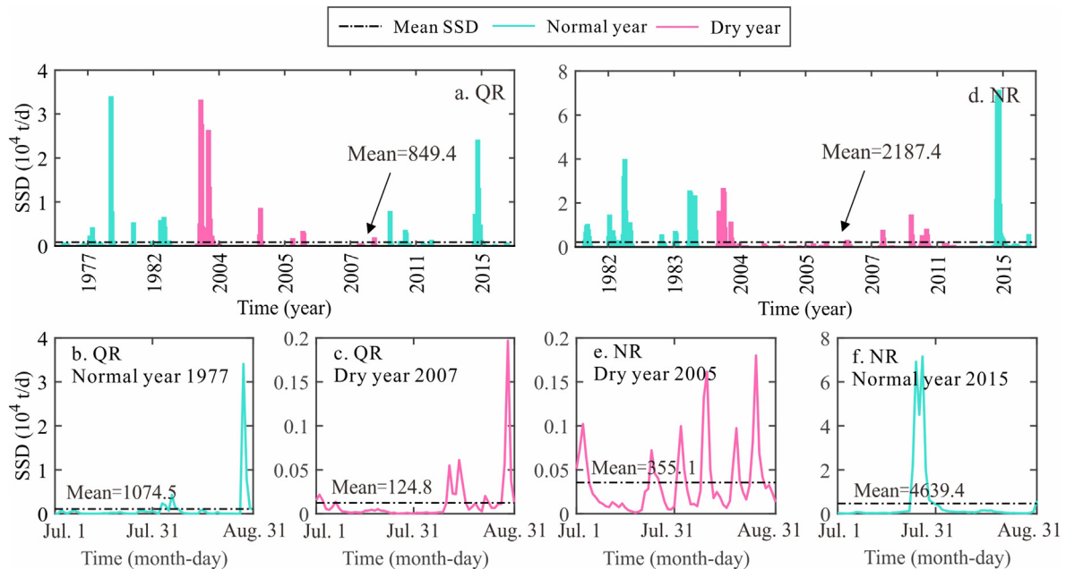
Fig. 4. Variations in daily SSDs in July and August of each non-TC year. SSDs of different hydrological years in plots (a)–(f) are shown in different colors. Plots (b), (c), (e) and (f) represent the changes in daily SSDs in July and August of specific normal and dry years. Due to the lack of daily SSD, the variations of SSD in the flood non-TC years are not shown in this figure.
