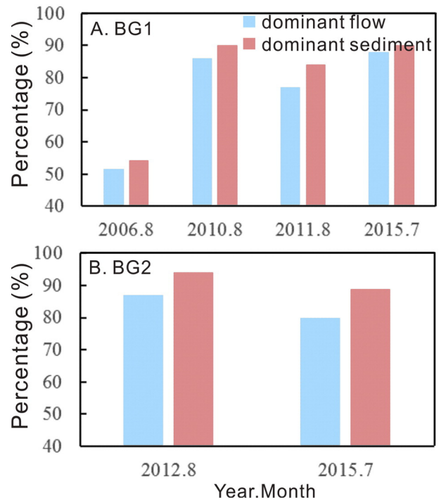
Fig. 13. A) The coefficient of dominant flow and sediment during the flood season at the BG1 station; B) the coefficient of dominant flow and sediment during the flood season at the BG2 station.
