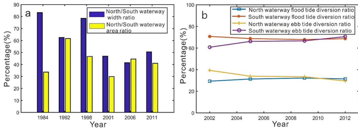
Fig. 12. a The width and area ratios of the Baimao Shoal North/South Waterway; b The flood and ebb tide diversion ratio of the North and South Waterways.
