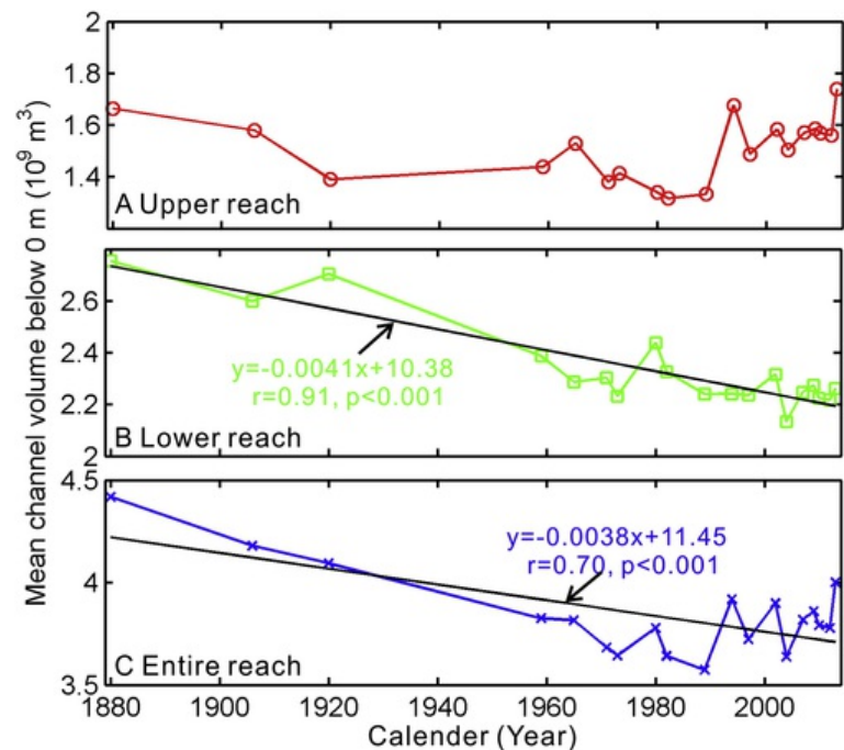
Fig. 4 Yearly variation of channel volume below 0 m isobath, with A) the upper reach; B) the lower reach; C) the entire reach.
