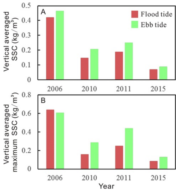
Fig. 11 A) Vertical averaged SSC during flood and ebb tides at the BG1 station; B) Vertical averaged maximum SSC during flood and ebb tides at the BG1 station.
