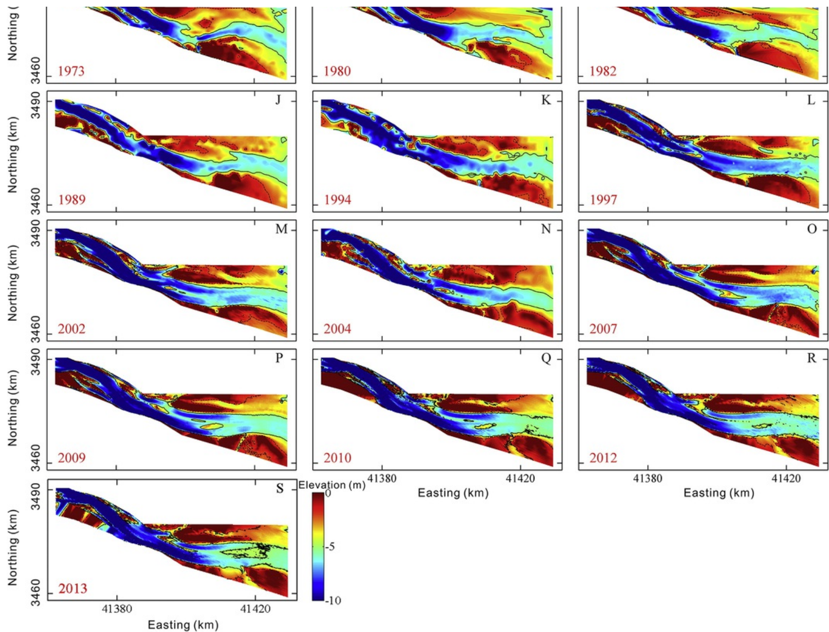
Fig. 2 Bathymetric maps of the North Channel over the period 1880 to 2013. alt-text: Fig. 2
