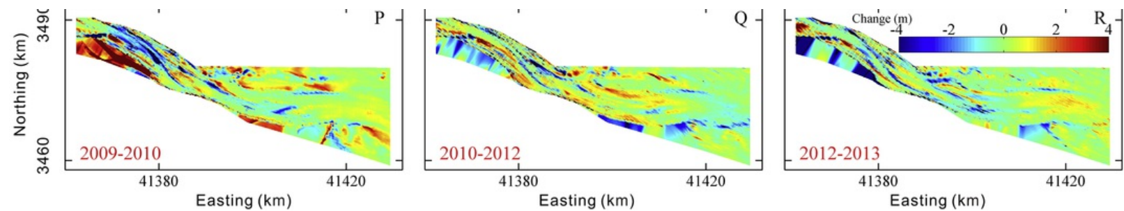
Fig. 6 Yearly erosion/deposition patterns of the North Channel at un-uniform intervals from 1880 to 2013.
