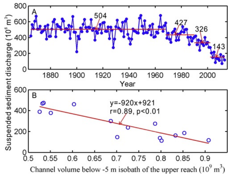
Fig. 10 A) Yearly suspended sediment discharge (SSD) into the Changjiang Estuary; B) the relationship between SSD and channel volume of the upper reach.
