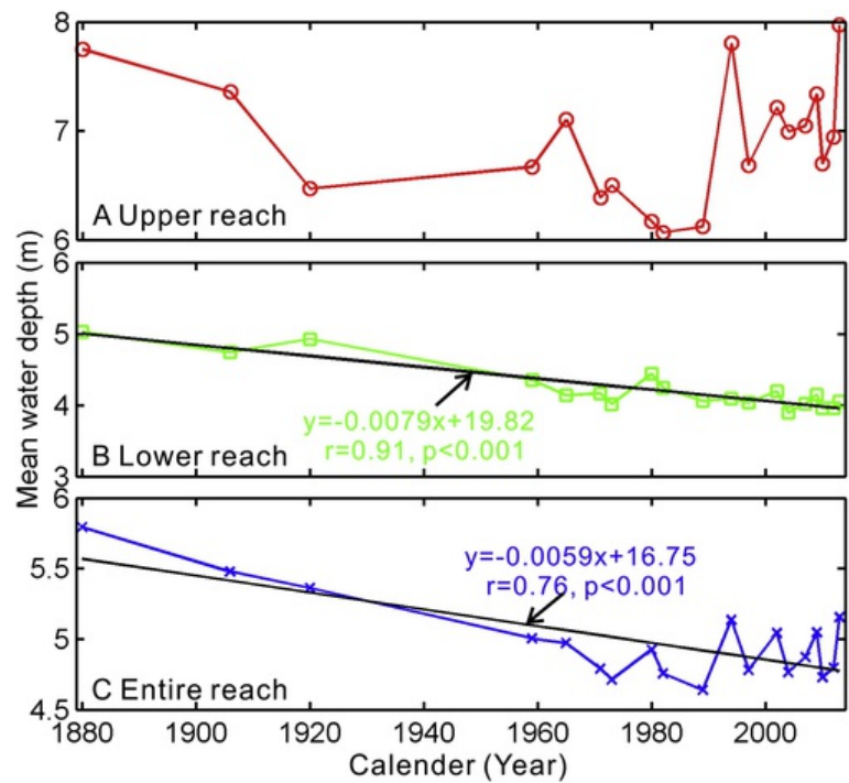
Fig. 3 Yearly variations of mean water depth, for A) upper reach; B) lower reach; C) the entire reach.
