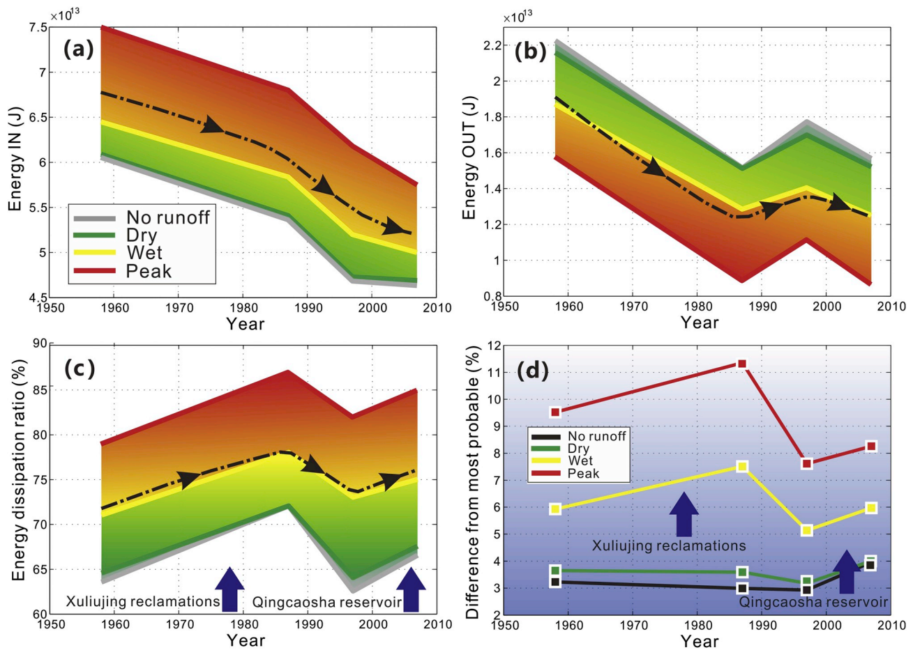
Fig. 7. Variation in the energy into and out of the South Branch of the estuary and the associated dissipation ratio and percentage difference from the most probable state over the studied period and for the different flow conditions examined.
