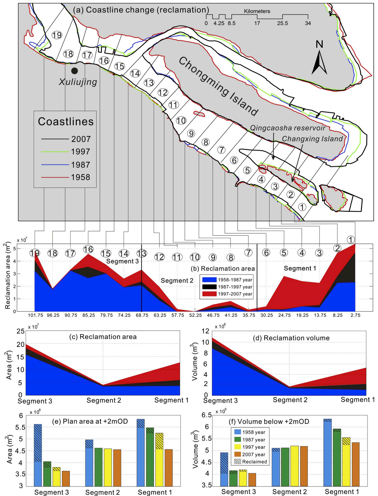
Fig. 4. (a) and (b) historical coastline changes and along-channel reclamation area variation derived from archived remote sensing images and navigation charts, (c) and (d) reclamation area and reclamation volume change over time for the three segments, and (e) and (f) the water area and volume relative to +2mOD. The shaded area of the bars is the area or volume removed due to reclamation that had occurred by the time of the subsequent survey.
