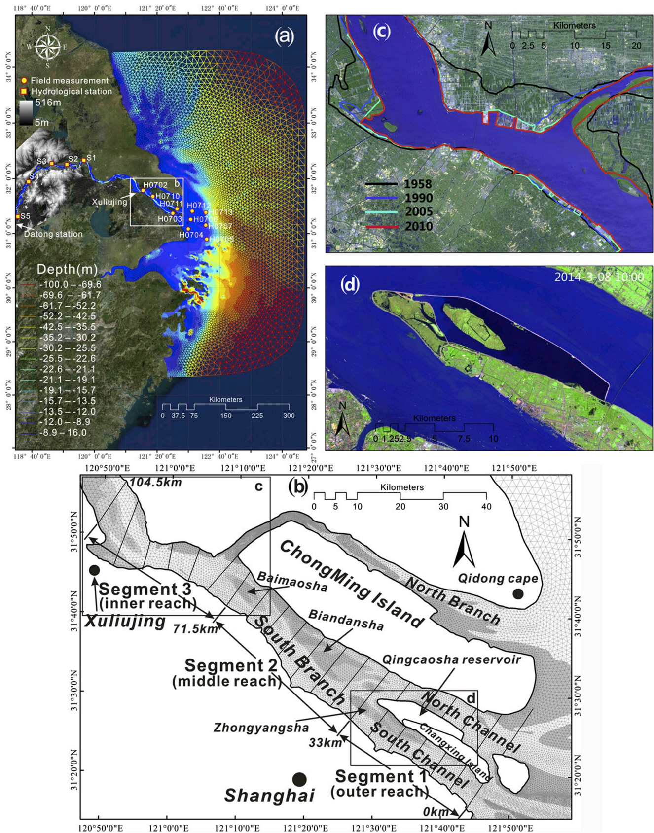
Fig. 1. (a) Sketch map of the triangular mesh for the entire modeling area in 2007, enlarged view at (b) the South Branch showing the 2007 shoreline, position of 5.5 km cross-sections and the 3 segment reaches, (c) remote sensing image at Xuliujing and historic changes in shorelines, and (d) recent remote sensing image of the Qingcaosha Reservoir.
