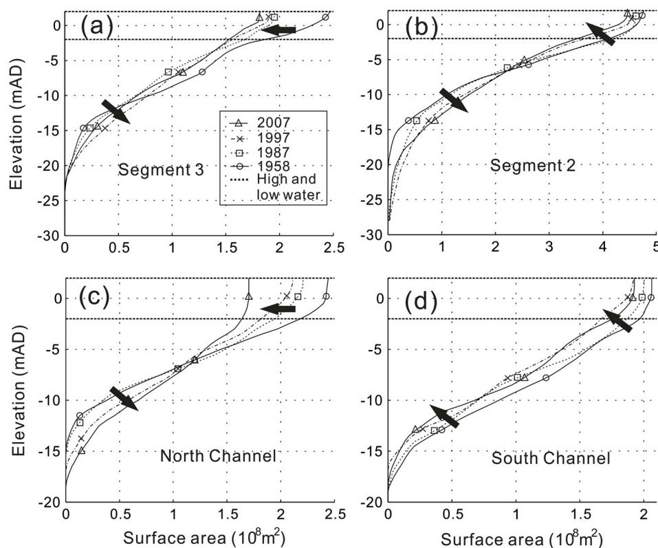
Fig. 3. Variation in hypsometry over time based on the 3 Segments, with the outer segment subdivided into the North and South Channels. The dotted horizontal lines represent high and low water levels, and the elevation is measured relative to the Huanghai1985 datum (mAD is meters above datum).
