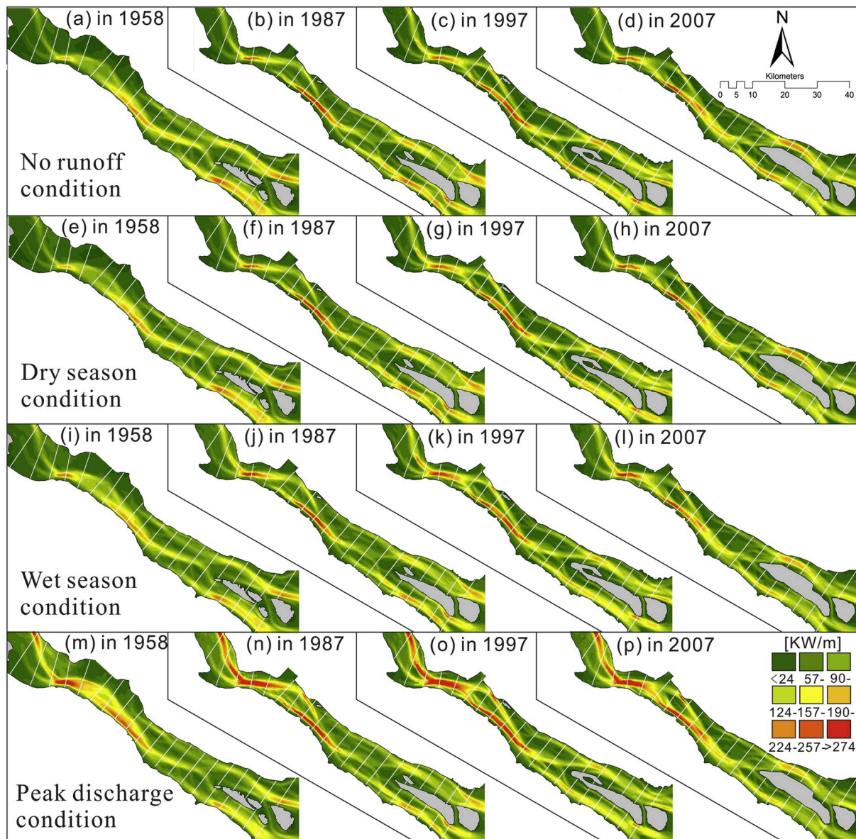
Fig. 5. Variation in tidally averaged energy flux per unit width in the South Branch of the Yangtze estuary under a range of flow conditions, showing variations over the studied period (1958–2007).
