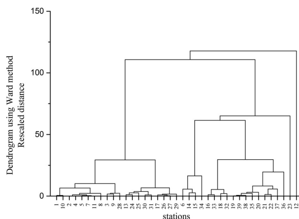
Figure 5. Cluster analysis of different stations represented by the same number as Table 1.
