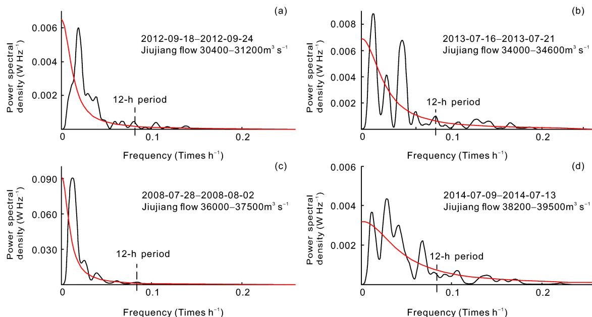
Figure 7 Water level spectrum analysis at Pengze station, corresponding to during different flow rates at Jiujiang station.
