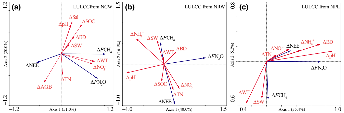
FIGURE 5 Redundancy analysis of the relationship between \Delta GHG (greenhouse gas) fluxes and \Delta EFs (environment factors) when the natural coastal wetlands (NCWs: a), riparian wetlands (NRWs: b), and peatlands (NPLs: c) were converted to the associated land-use/land-cover change (LULCC) types [Colour figure can be viewed at wileyonlinelibrary.com ]
