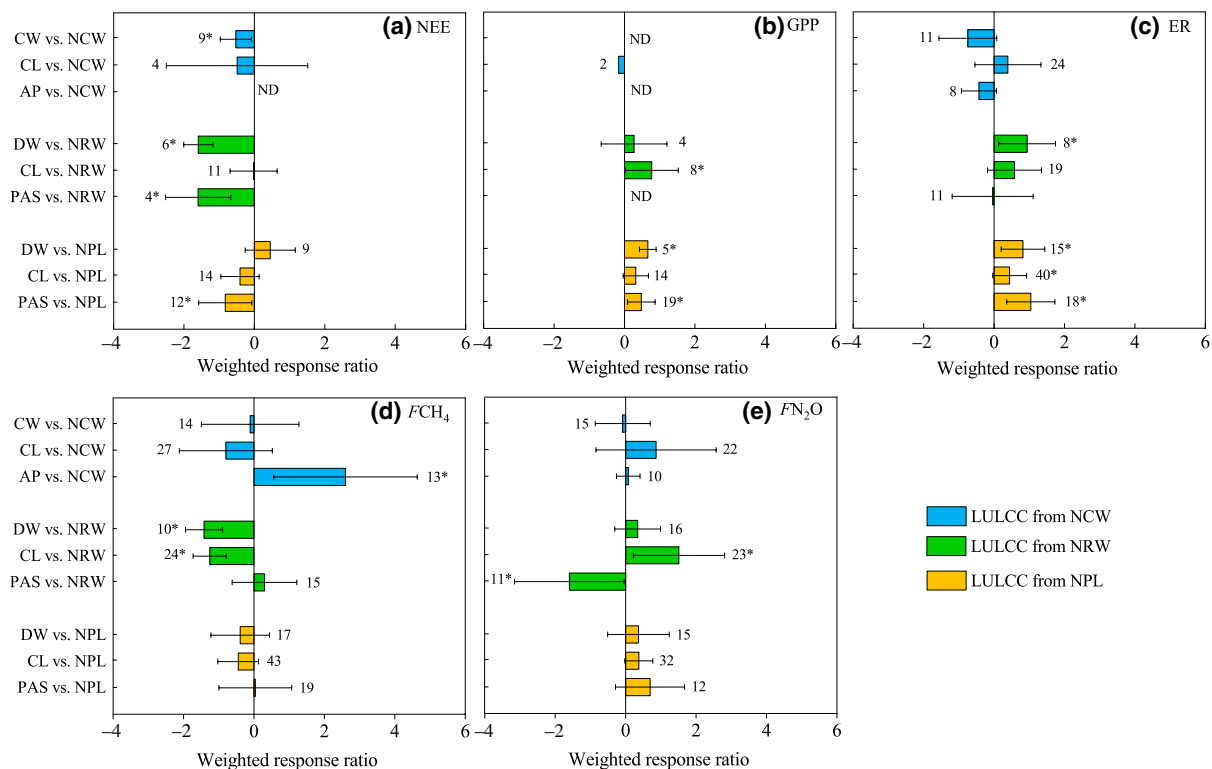
FIGURE 3 Weighted response ratios (RR ++ ) of (a) net ecosystem CO 2 exchange (NEE), (b) gross primary productivity (GPP), (c) ecosystem respiration (ER), (d) methane fluxes (FCH 4 ), and (e) nitrous oxide fluxes (FN 2 O) to the land-use/land-cover change (LULCC) types from natural wetlands. Bars represent the RR ++ values and 95% CIs. If the 95% CI value of RR ++ did not overlap with zero, the LULCC response was considered significant. Vertical lines were drawn at RR = 0. The sample size for each variable is shown next to the bar, and asterisks (*) denote significance at p < .05 . ND, no data [Colour figure can be viewed at wileyonlinelibrary.com ]
