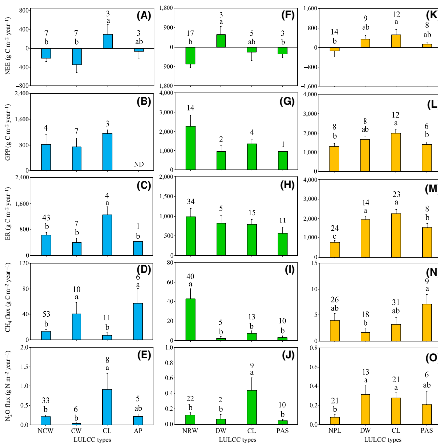
FIGURE 2 Changes in greenhouse gas fluxes in the natural coastal wetlands (NCWs) and the associated LULCC types (A-E), the natural riparian wetlands (NRWs) and the associated LULCC types (F-J), and the natural peatlands (NPLs) and the associated LULCC types (K-O). The sample size for each variable is shown next to the bar, and different lowercase letters denote significance at p < .05 . ND, no data [Colour figure can be viewed at wileyonlinelibrary.com ]
