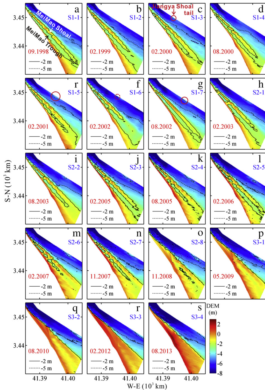
Fig. 3. Representative DEM and isobaths (−2 and −5 m) of the NHS for 3 stages, with a–g) showing Stage 1, h–o) showing Stage 2 and p–s) showing Stage 3. Obviously, the Meimao Trough had long and complete form in Stage 1, became disrupted in Stage 2 and disappeared in Stage 3. The red circle marks stretching of the Jiangya Shoal's tail within the study area during Stage 1, with the solid circle indicating the significant stretching of Jiangya Shoal's tail and the dashed circle indicating the slight stretching of the Jiangya Shoal's tail.
