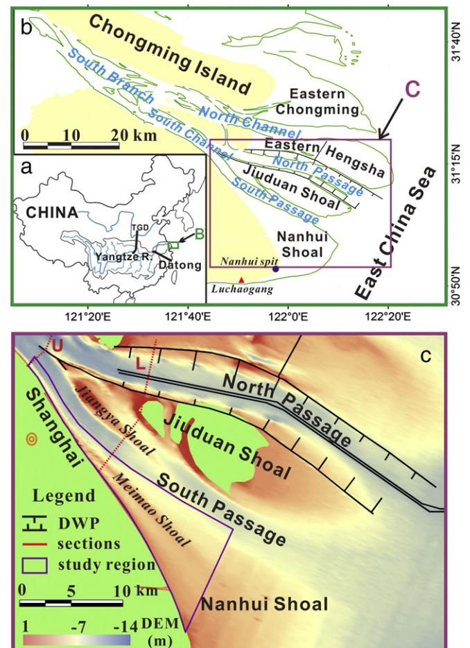
Fig. 1. Maps of a) China, which shows the drainage basin of the Changjiang River and the locations of the Three Gorges Dam and Datong station; b) geographic setting of the Changjiang estuary, including the Nanhui Shoal, South Passage, and Luchaogang gauge station; and c) landform of the Nanhui Shoal that was surveyed in 2002, which shows the locations of the Jiangya Shoal, Meimao Shoal, Deep Waterway Project, configurations of the study region, and sections for calculating the ebb flow diversion ratios.
