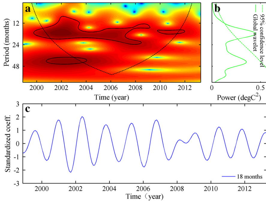
Fig. 7. Wavelet analysis of the NHS's volume changes between surveys: (a) contoured coefficient, (b) global wavelet coefficient, and (c) time series of the periodic component (namely 18 months) extracted from (a).
