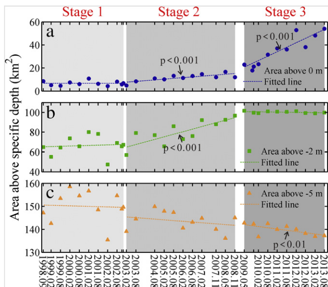
Fig. 6. Area changes of NHS a) above 0 m, b) above -2 m and c) above -5 m. The three stages are depicted by gradually deepening color areas, with the fitting line shown.
